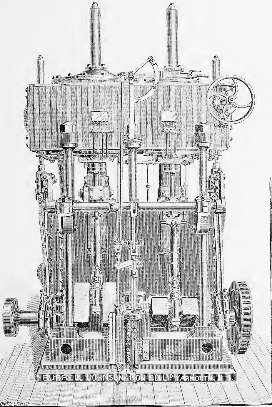
TANDEM COMPOUND SURFACE CONDENSING ENGINE OF THE STEAMER WEYMOUTH.
